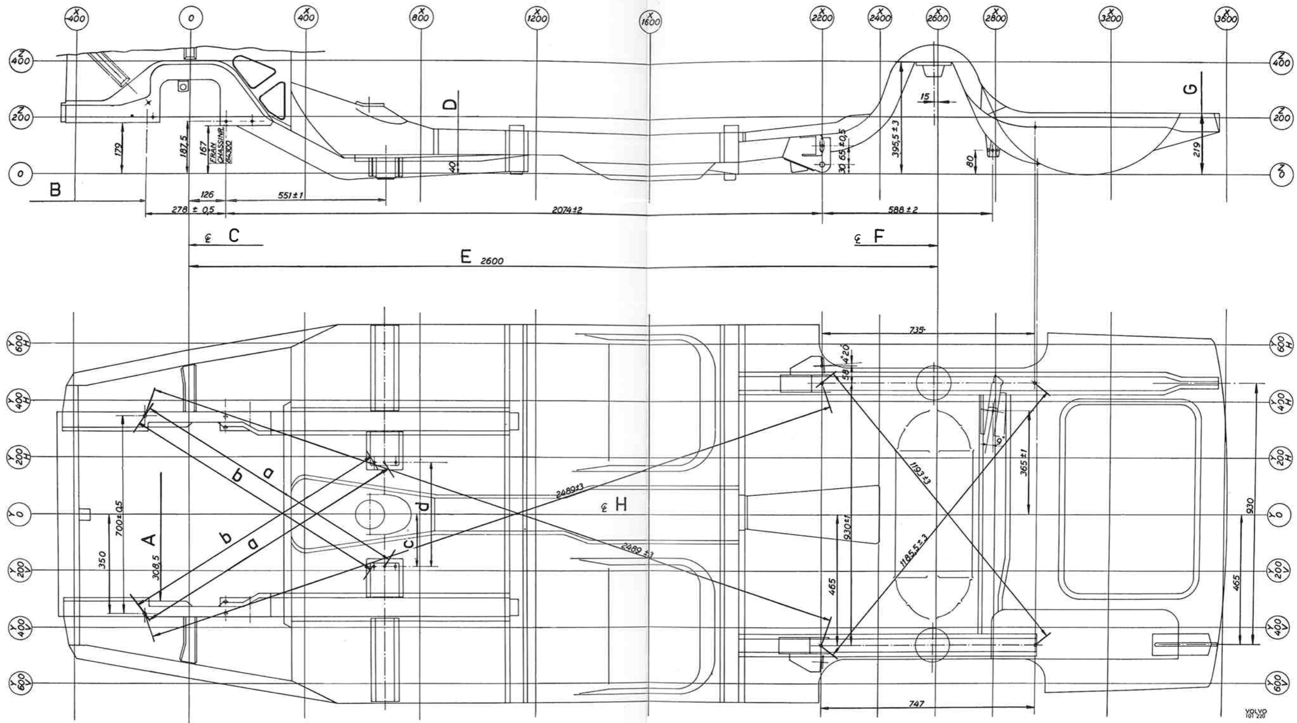
Illustration A. Control drawing for body floor, P 120 (2- and 4-door)
