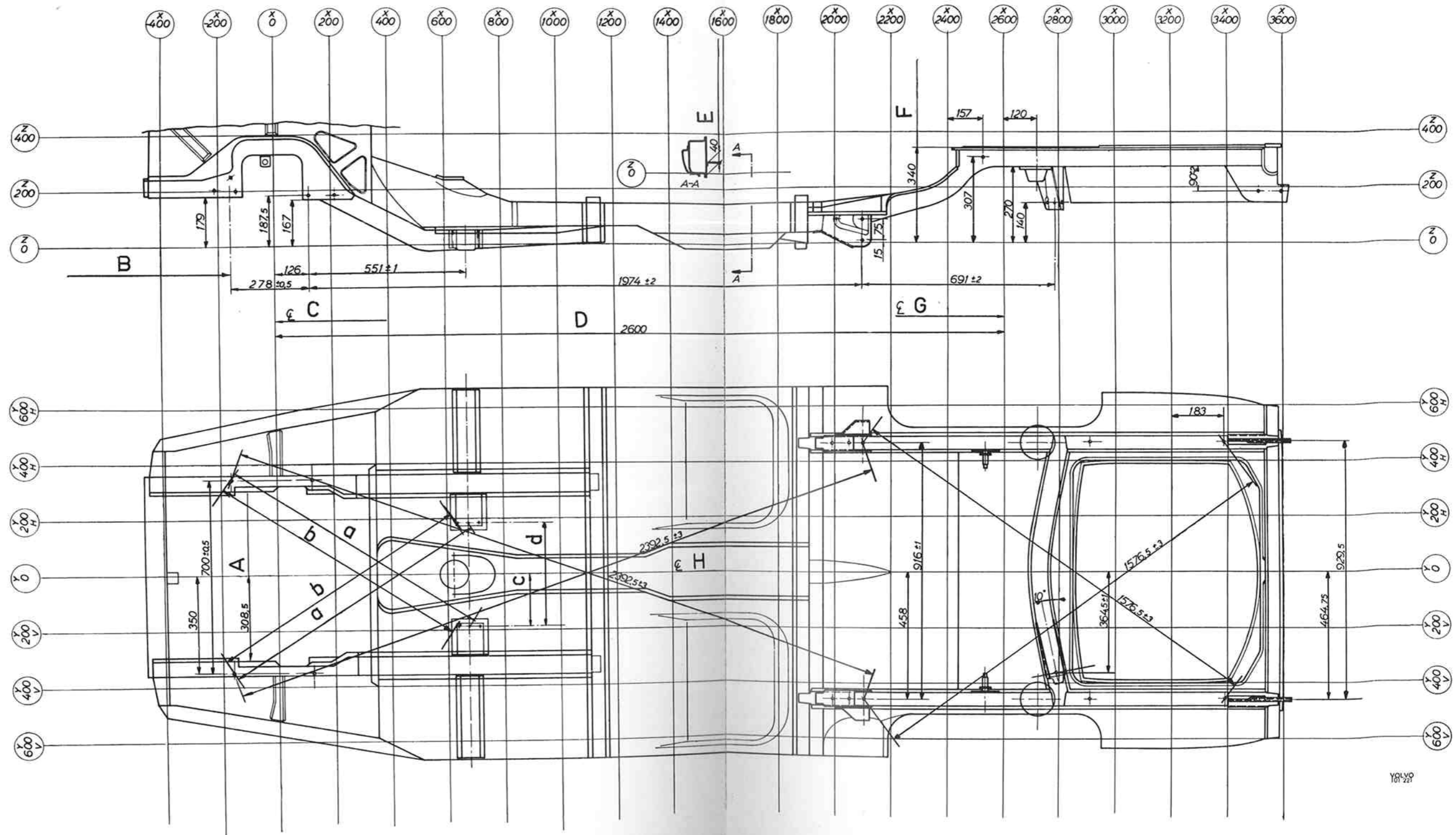
Illustration B. Control drawing for body floor, P 120 Station Wagon
