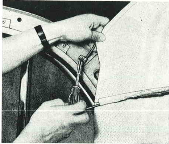
Fig. 73. Fitting rear clip
