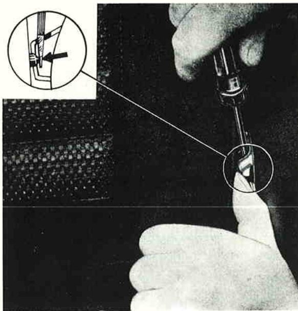
Fig. 65. Releasing catch for removing rear seat backrest on Station Wagon
