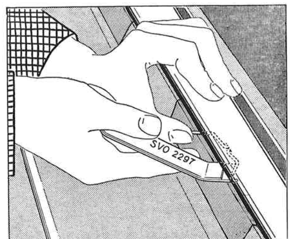
Fig. 52. Fitting spring
