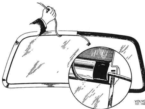
Fig. 56. Fitting trim moulding
