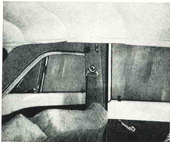
Fig. 75. Headlining ready for stretching
