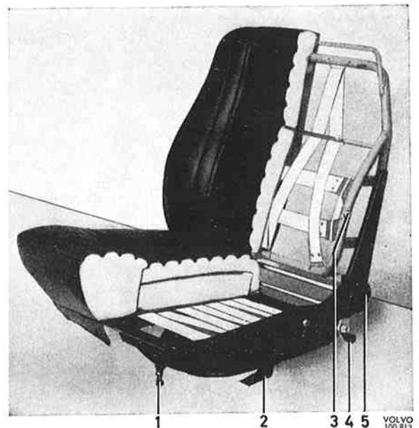
Fig. 64. Front seat
