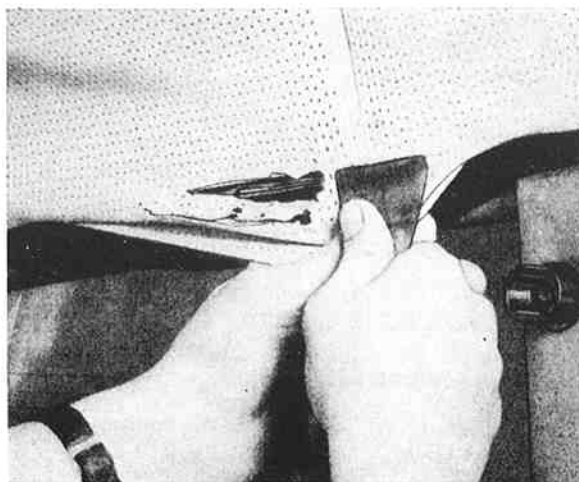
Fig. 69. Stretching the headlining
