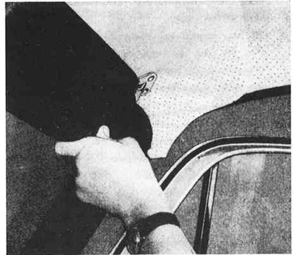
Fig. 71. Fitting sun visor
