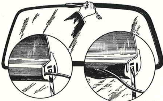
Fig. 61. Fitting windscreen
